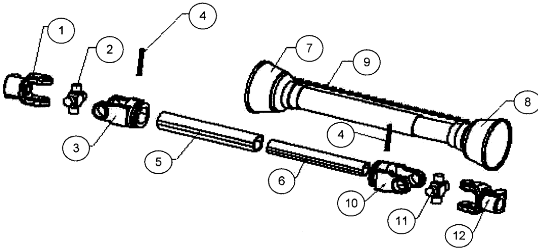
LS309 - SPLINE TO ROUND (TRACTOR TO ROUND BAR)
